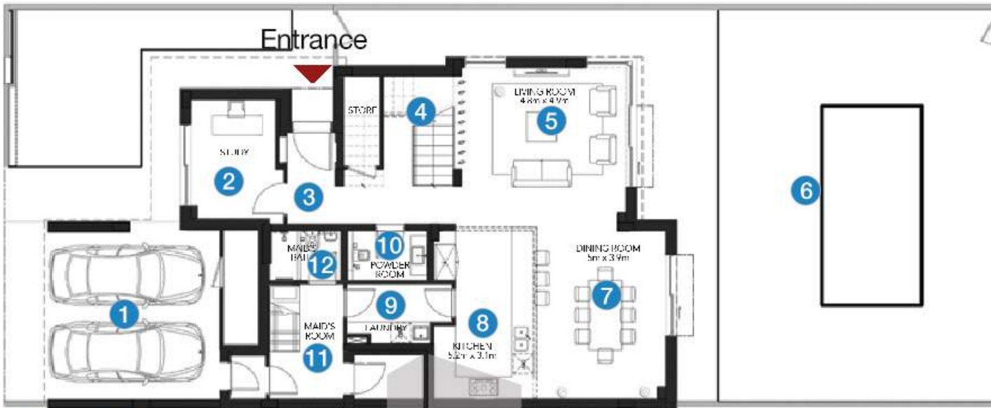
Ground Floor
